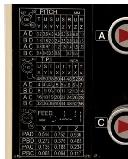
Thread-Feed Chart
