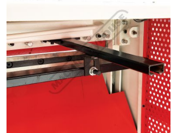
Rear Back Gauge
