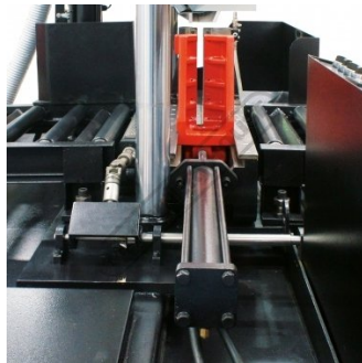
Full Stroke Hydraulic Vice
