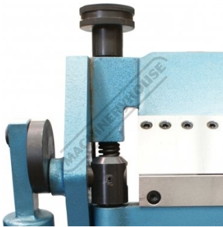
Material Clamping Tension Adjustment Dial
