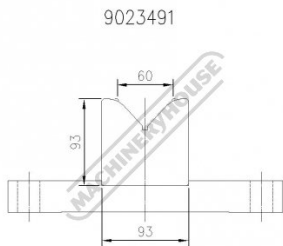
Single Vee Pressbrake Diagram
