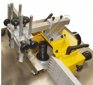
Cutter Guard with Dust Chute
