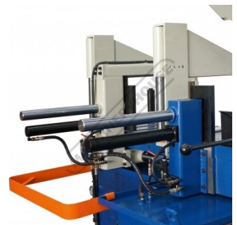
Full Stroke Hydraulic Vice Clamps
