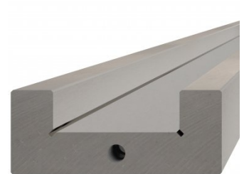
S997B 60mm Die Rail Pressbrake Tooling
