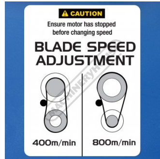
Belt Speed Diagram
