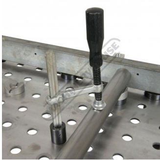
Shown Clamping Round Material
