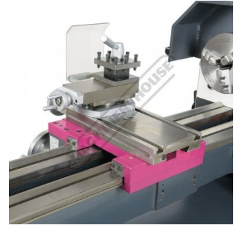
Saddle Rear View
