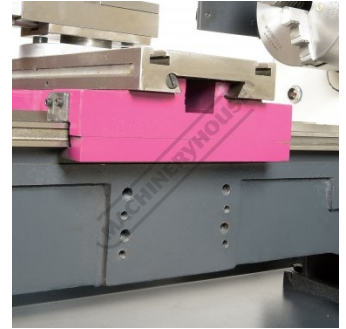
Mounting Point for Optional Milling Head
