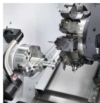
LYNX 2100LY
