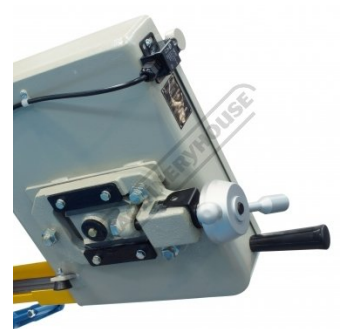
Blade Tension Mechanism
