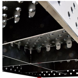
Stengthened by Welded Webbing
