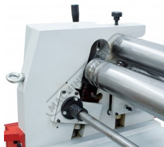
Motorised Up and Down Rear Curving Roller Left Side
