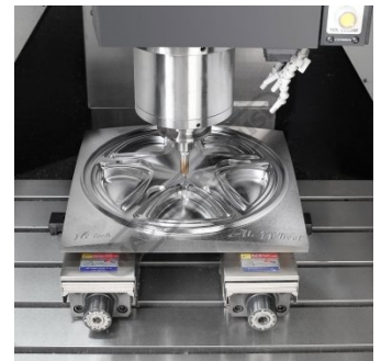
DNN650II Milling
